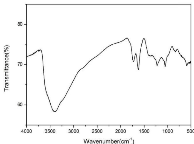
FTIR pattern of graphene oxide powder
