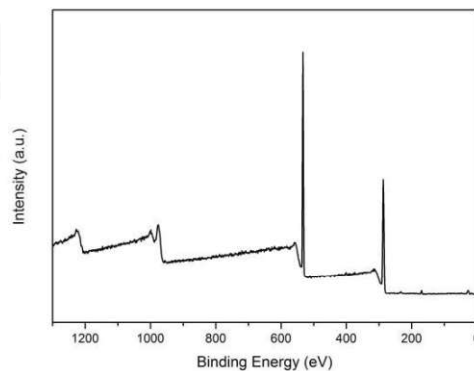
XPS spectrum of graphene oxide sheet
