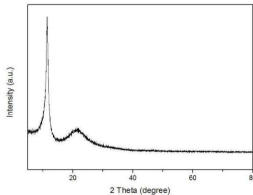
XRD pattern of graphene oxide sheet
