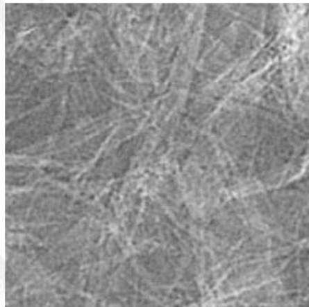
TEM of graphene oxide water dispersion (<500 nm)
