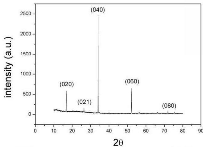
XRD pattern of black phosphorus crystal
