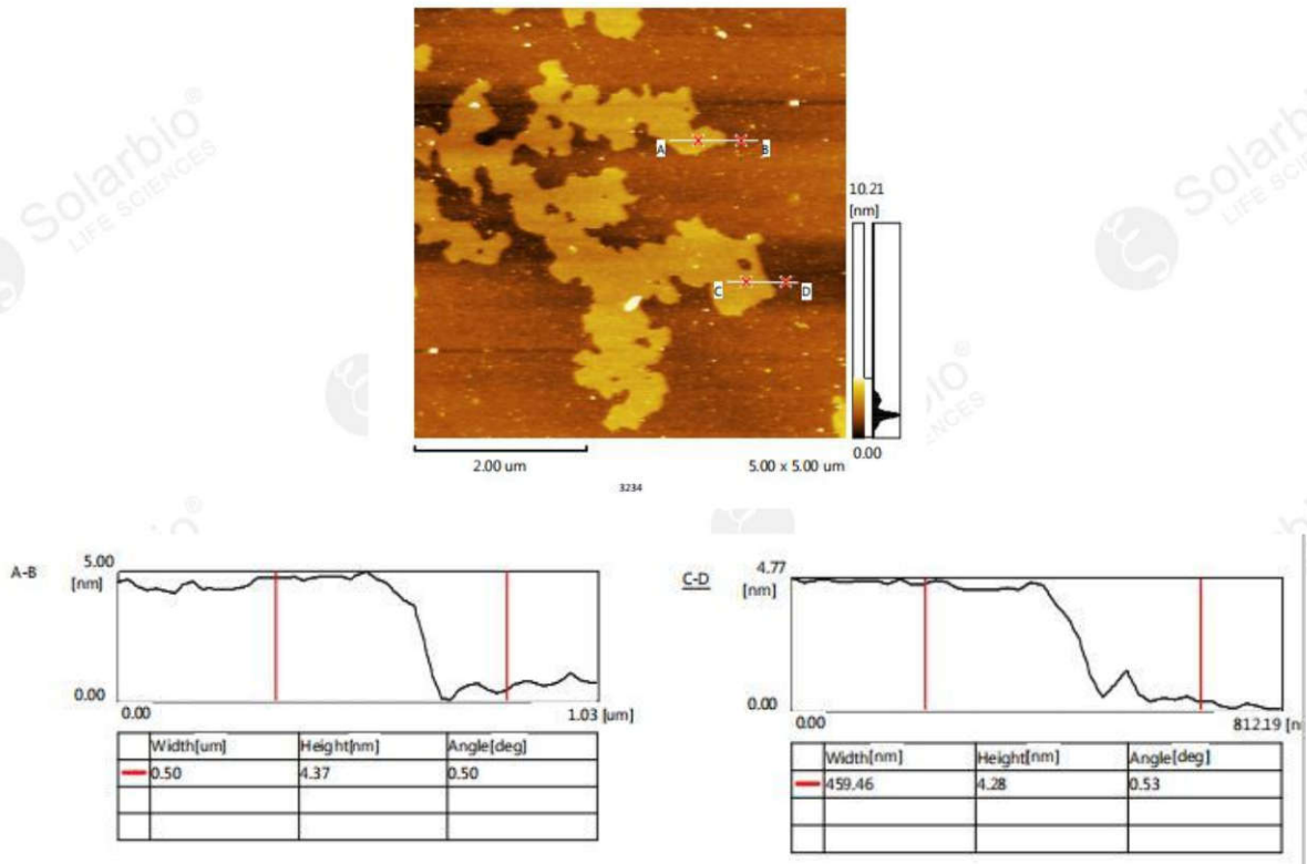
AFM image of Thin Layer WS 2 Dispersion
