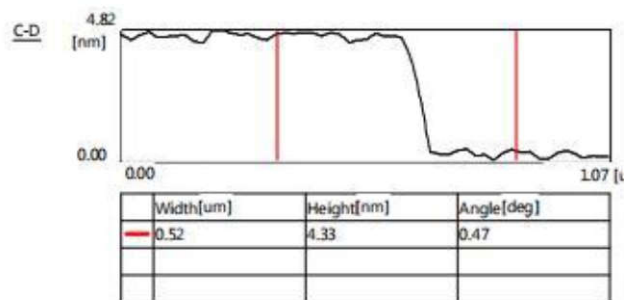
AFM image of Thin Layer Nano WS2 Dispersion
