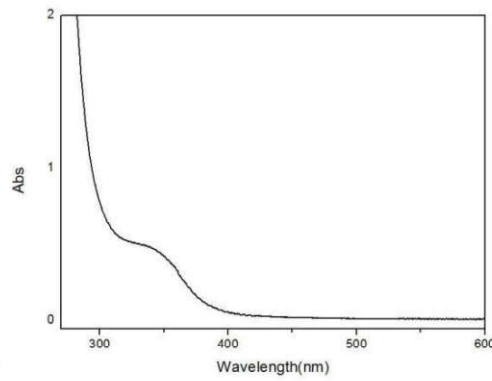
Absorption spectrum of GO quantum dots powder dispersed in water
