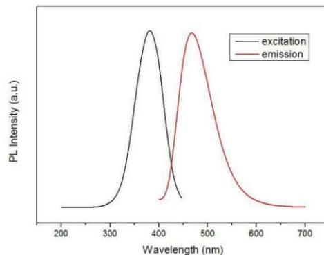
PL spectrum of GO quantum dots powder dispersed in water
