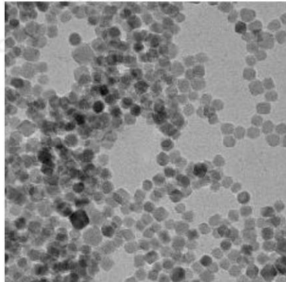
TEM image of DMSA Coated Fe 3 O 4 Nanoparticles (7nm)
