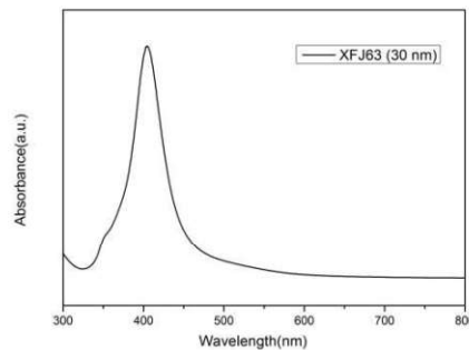
UV absorption spectrum of Ag Nanoparticles (30nm)
