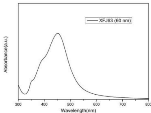
UV absorption spectrum of Ag Nanoparticles (60nm)
