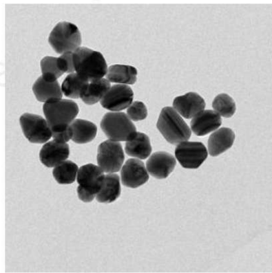
TEM of Ag Nanoparticles (90nm)
