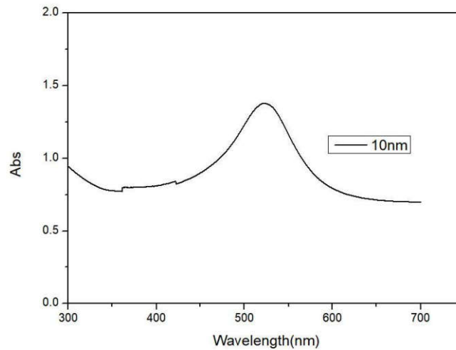
UV - Visible absorption spectrum of Au Nanoparticles (10nm)
