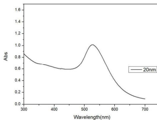
UV - Visible absorption spectrum of Au Nanoparticles (20nm)
