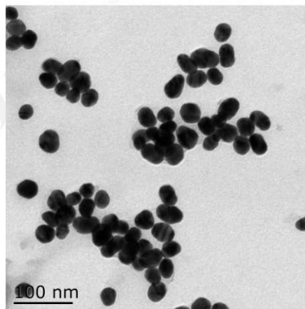
TEM image of Au Nanoparticles (30nm)
