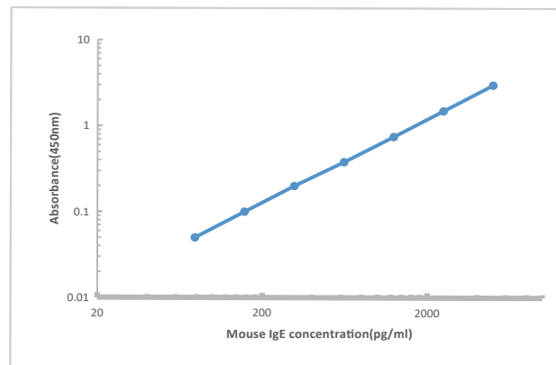
Representative standard curve for Mouse IgE ELISA.
